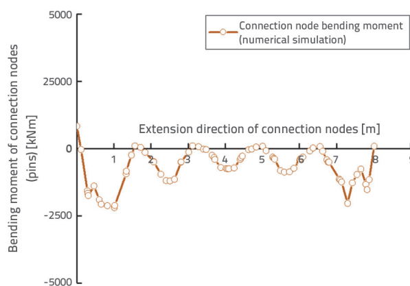
Figure 13. Finite element simulation of connection node in bending moment in direction of extension
