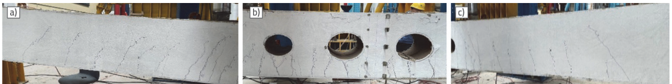
Figure 12. Final failure state of specimen PECB3: a) North side area; b) Mid-span region; c) South side area
