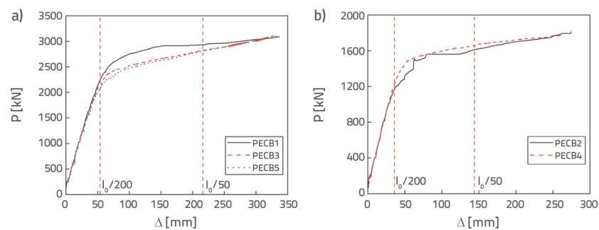
Figure 15. Load-midspan deflection curve: a) PECB1, PECB3 and PECB5; b) PECB2 and PECB4
