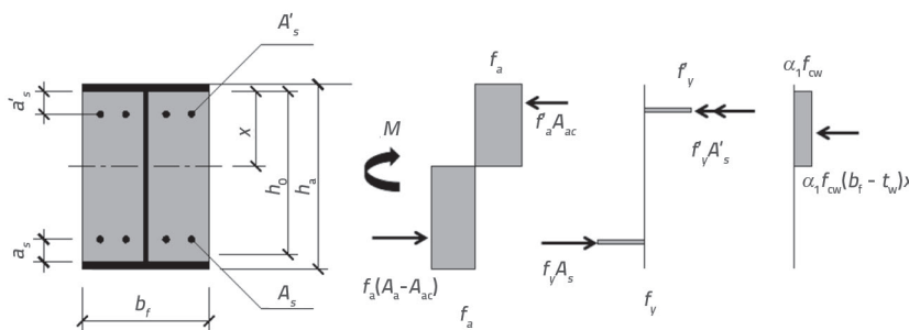
Figure 7. Section diagram and equivalent rectangular stress diagram of PEC beams
