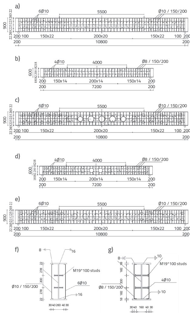
Figure 8. Schematic diagram of PEC beams: a) Specimen PECB1 elevation; b) Specimen PECB2 elevation; c) Specimen PECB3 elevation; d) Specimen PECB4 elevation; e) Specimen PECB5 elevation; f) Middle section of main beam span; g) Mid-span section of secondary beam
