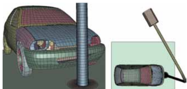
Figure 11. 3-D numerical modelling of vehicle and column [8]
